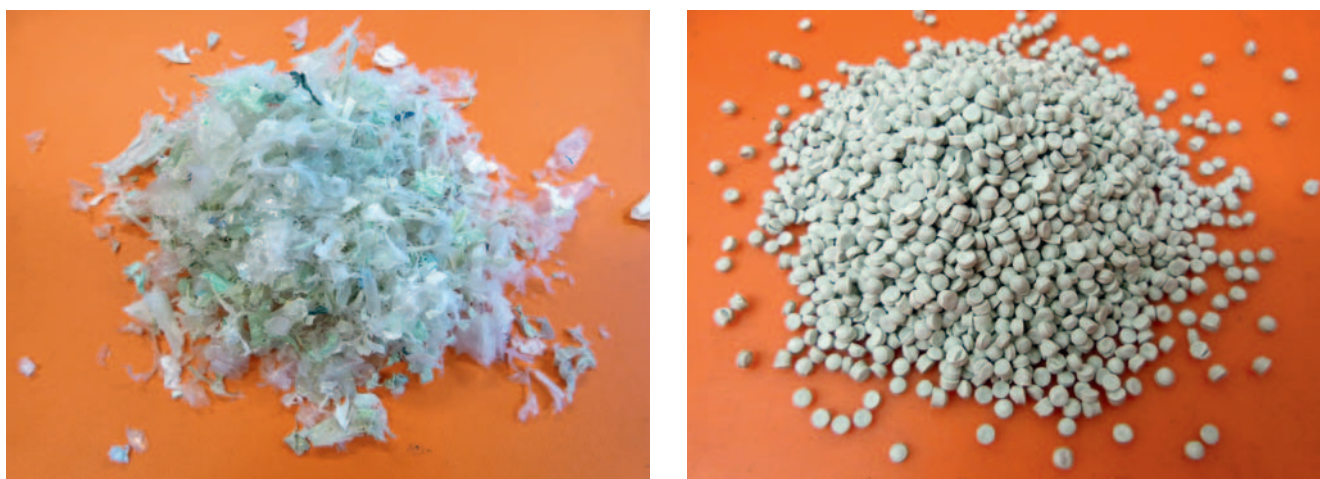
Figure 5. Washed shreds of severely contaminated agricultural film (left) processed with Corema 1108 T (filter system Erema SW 4/134 RTF, 300 µm) to make recycled pellets with 75 % CaCO 3 content
